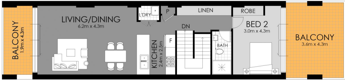
UPPER LEVEL
